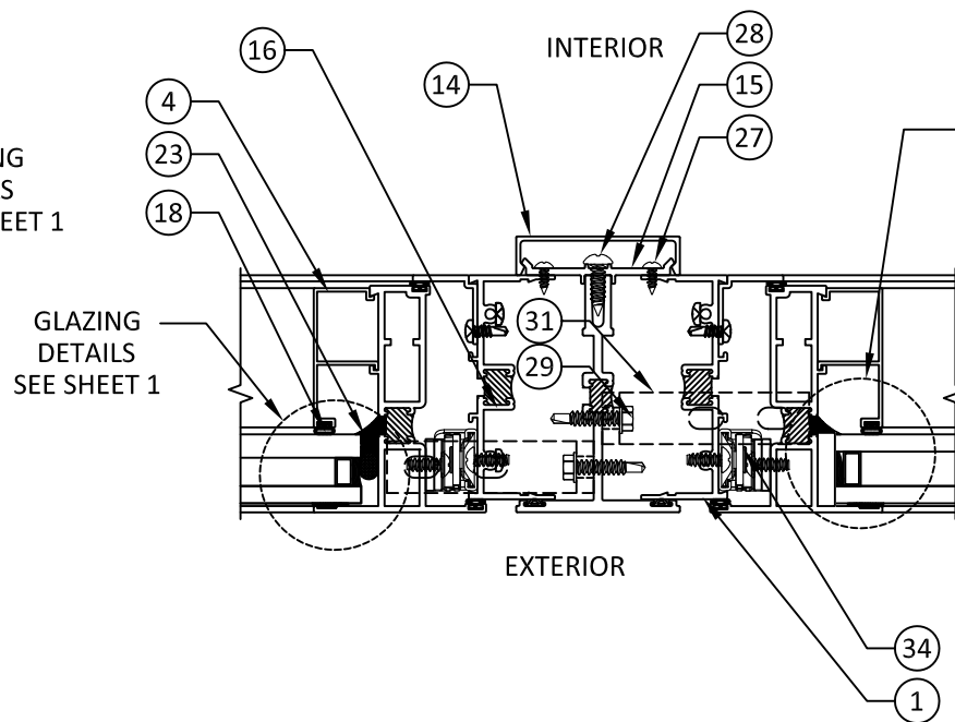
B 7 HORIZONTAL SECTION MULLION ( SPAN UP TO 72")
