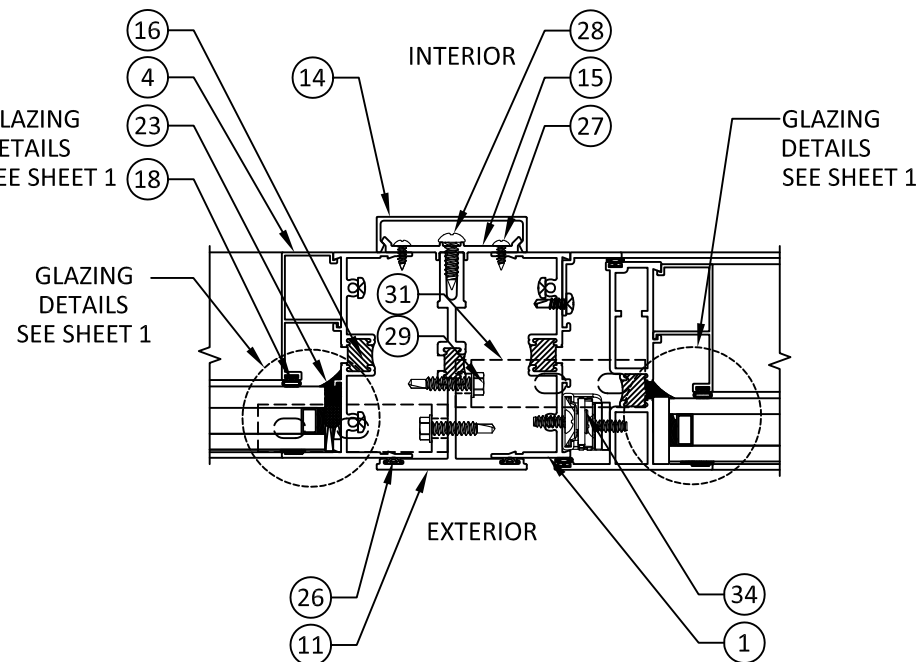
C 7 HORIZONTAL SECTION MULLION ( SPAN UP TO 72")
