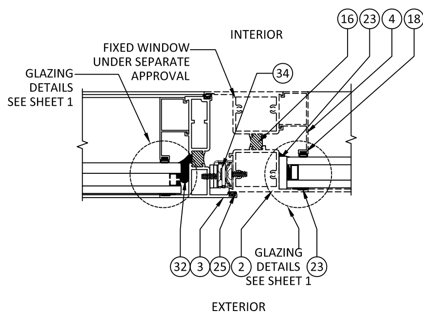
E 7 HORIZONTAL SECTION MEETING RAIL ( MAX SPAN 72")
