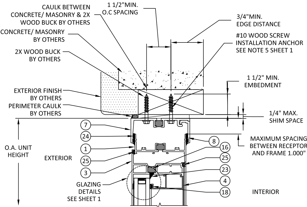
A 4 VERTICAL SECTION HEAD - 2X WOOD BUCK THROUGH FRAME INSTALLATION
