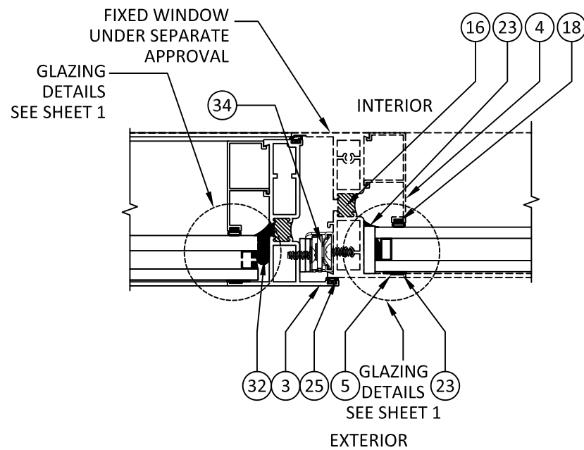
D 7 HORIZONTAL SECTION MEEETING RAIL ( MAX SPAN 60")
