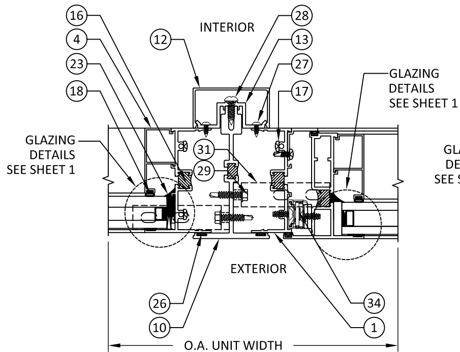
A 7 HORIZONTAL SECTION MULLION ( SPAN LONGER THAN 72")
