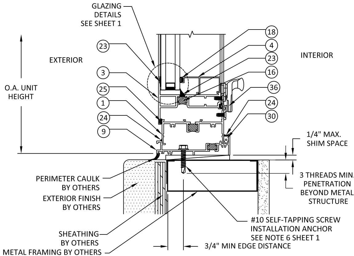
B 4 VERTICAL SECTION SILL - METAL STUD THROUGH FRAME INSTALLATION
