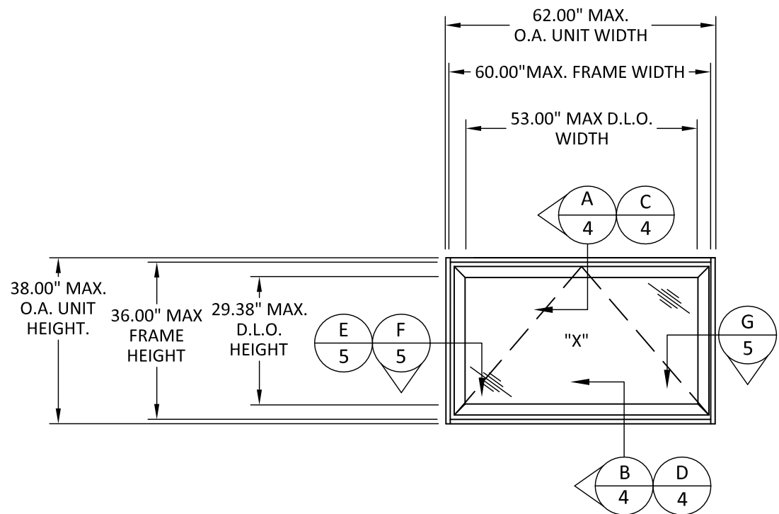
EXTERIOR ELEVATION PROJECT-OUT WINDOW
