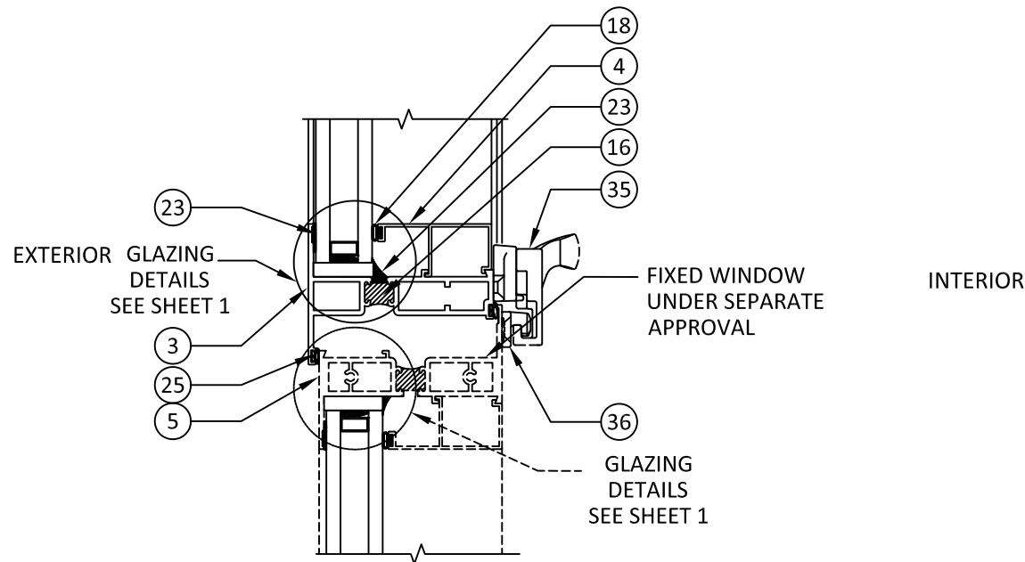
C 6 VERTICAL SECTION MEETING RAIL PO/FX ( MAX SPAN 60")
