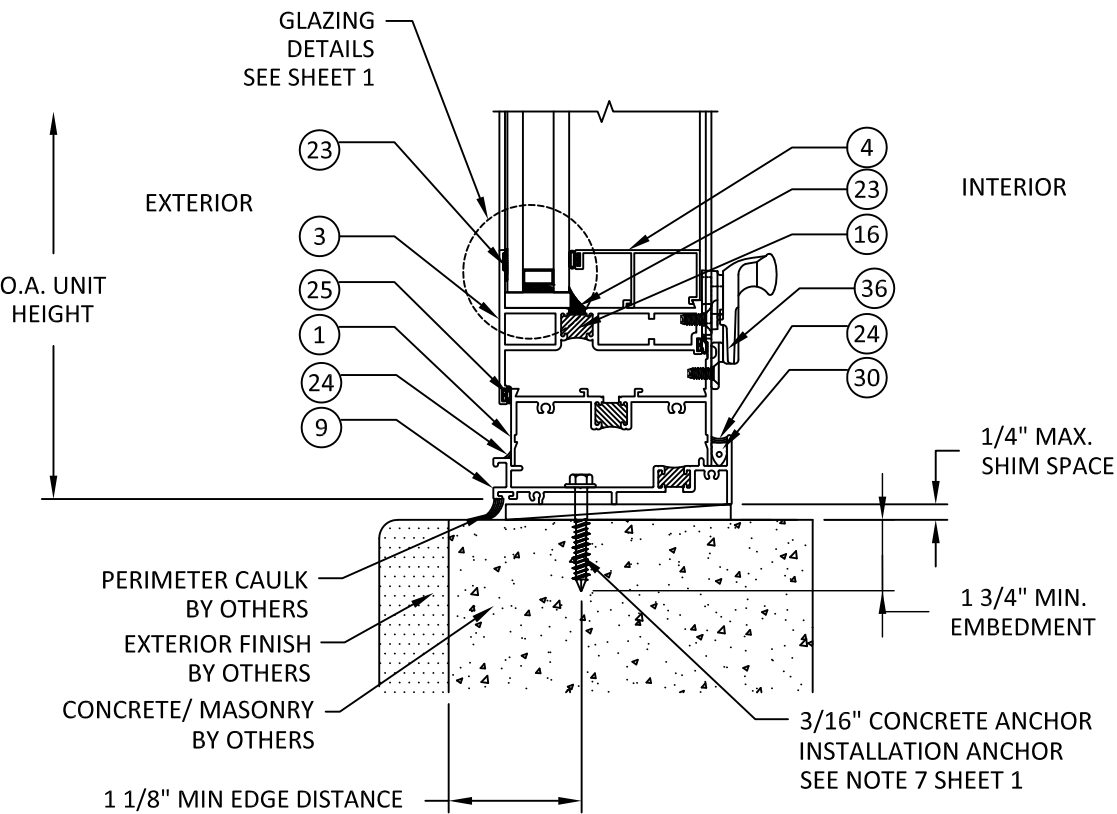
D 4 VERTICAL SECTION SILL - CONCRETE OR CMU THROUGH FRAME INSTALLATION
